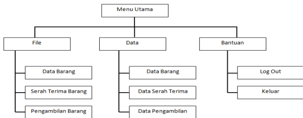
Figure 1. HIPO Chart
