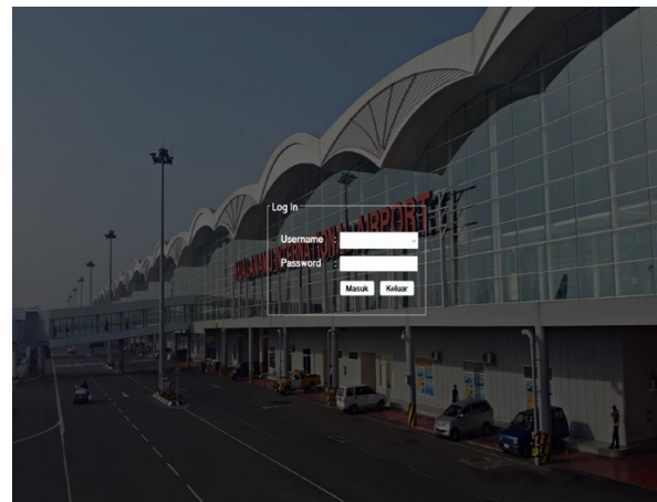
Figure 3. Login Form
