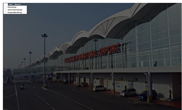
Figure 4. Main Form
